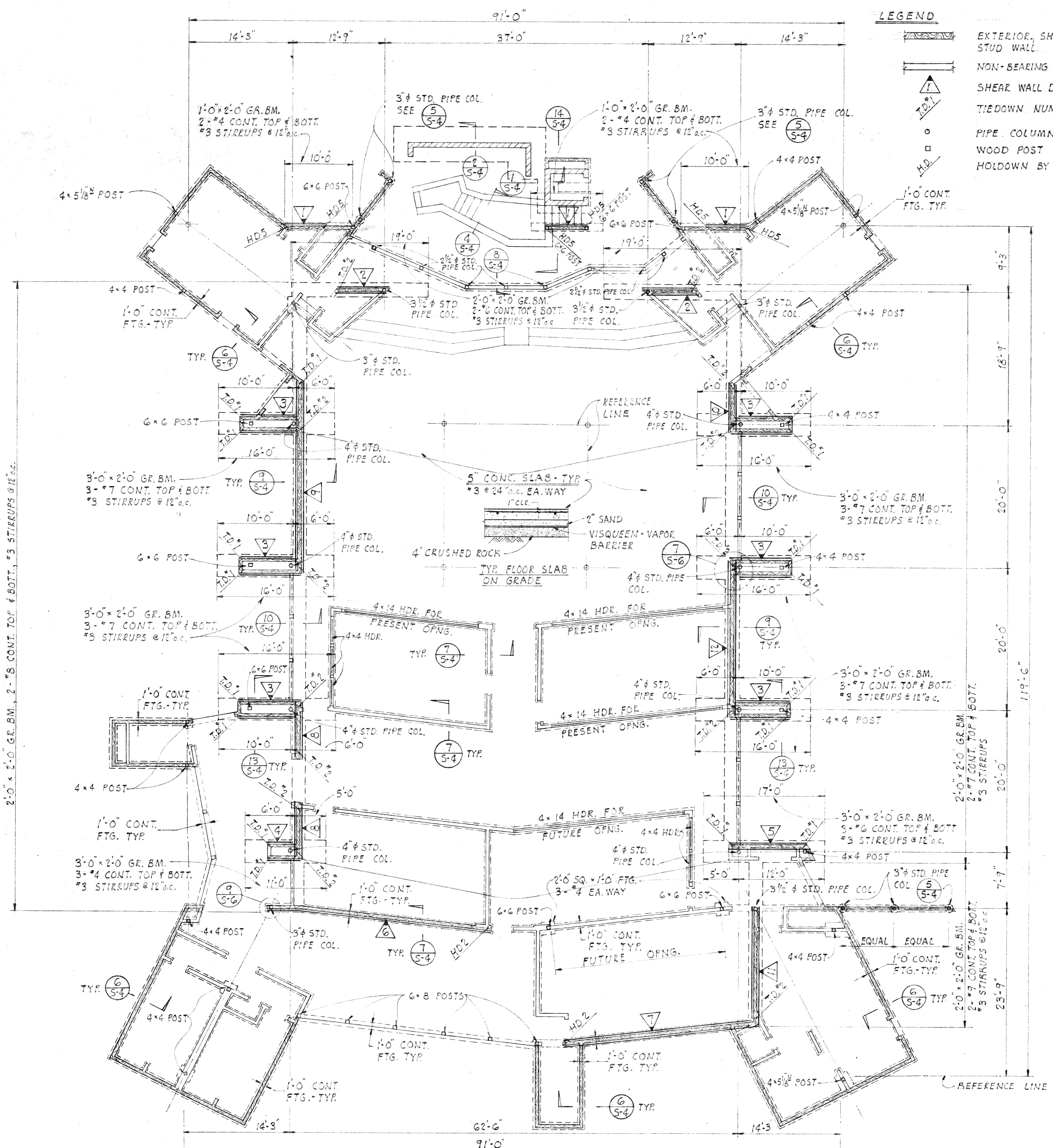
FOUNDATION PLAN
