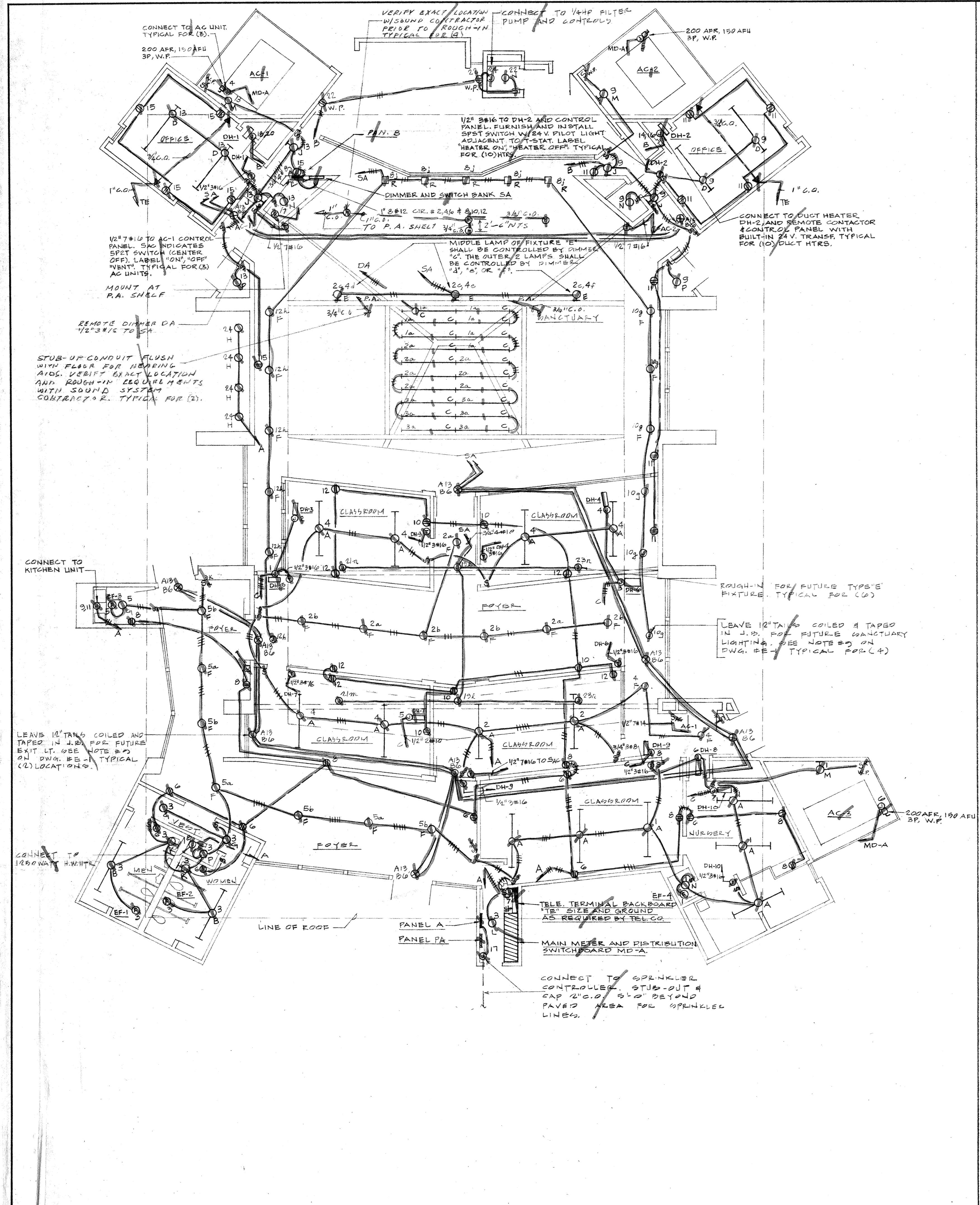
ELECTRICAL-LIGHTING & POWER PLAN SCALE 1/8"=1'-0"
