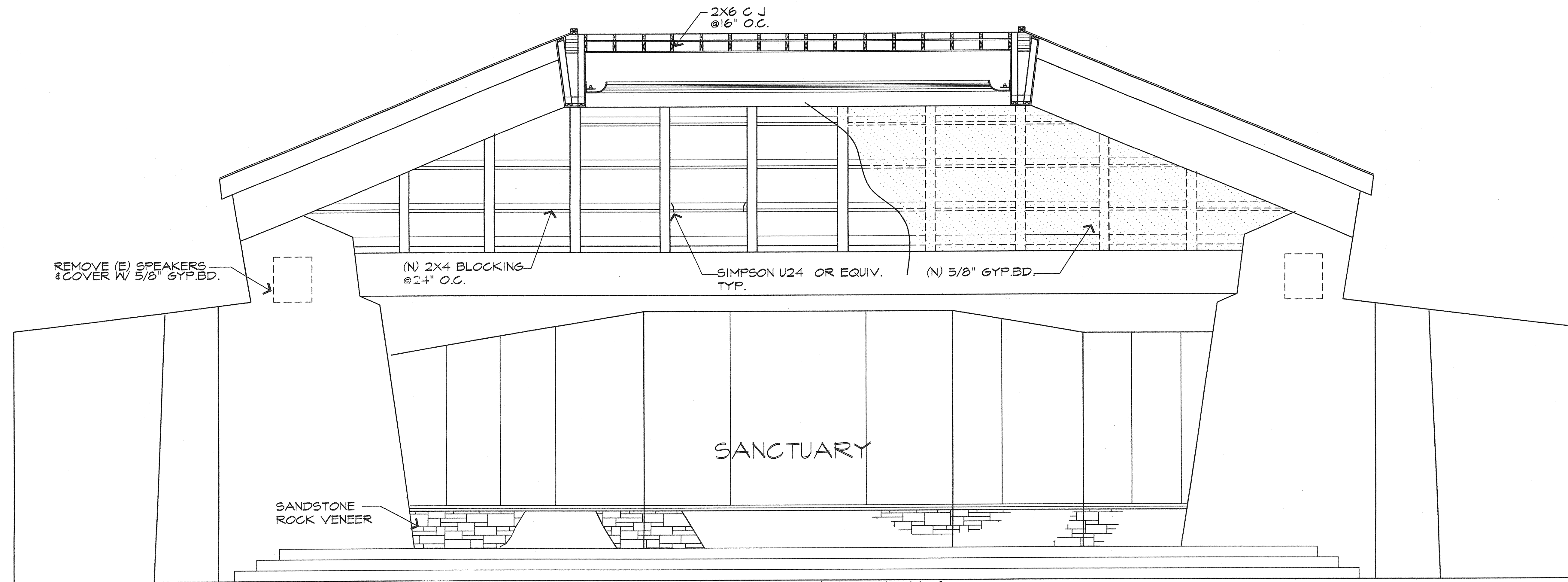
ELEVATION/SECTION A SCALE: 3/8"=1'-0"
