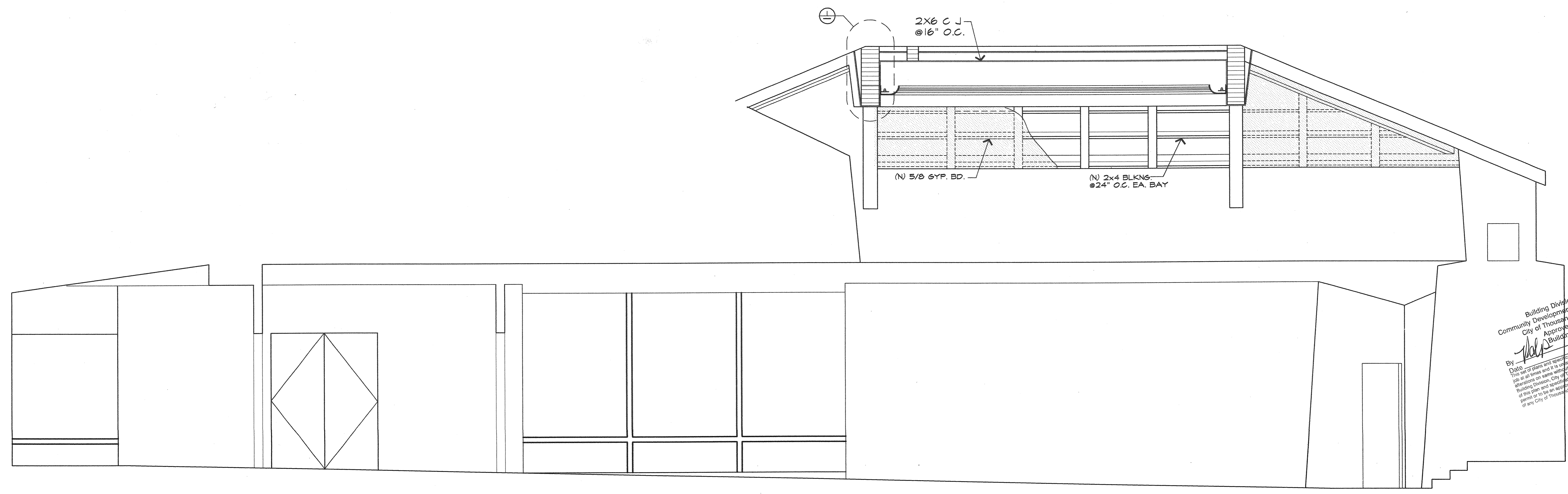
ELEVATION/SECTION C SCALE: 3/8"=1'-0"
